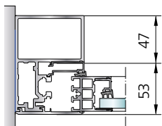
Jamb reinforced
